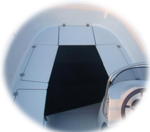
* sun deck / fishing deck 3 parts made of waterproof plywood with upholstery (console to the front)
